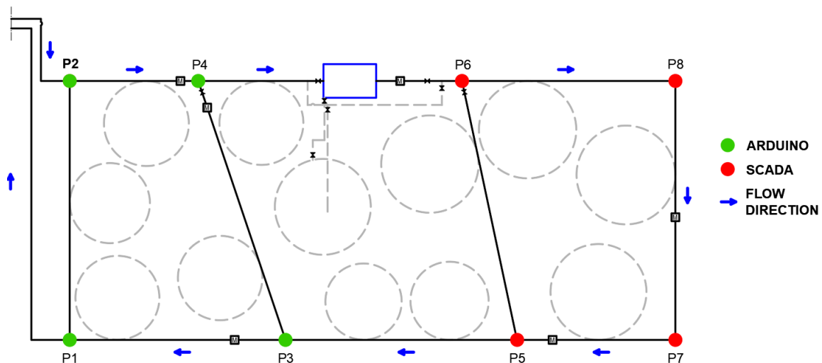
Figure 5. Network configuration.
